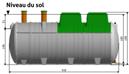
Tricel Seta Simplex FR5/4100
